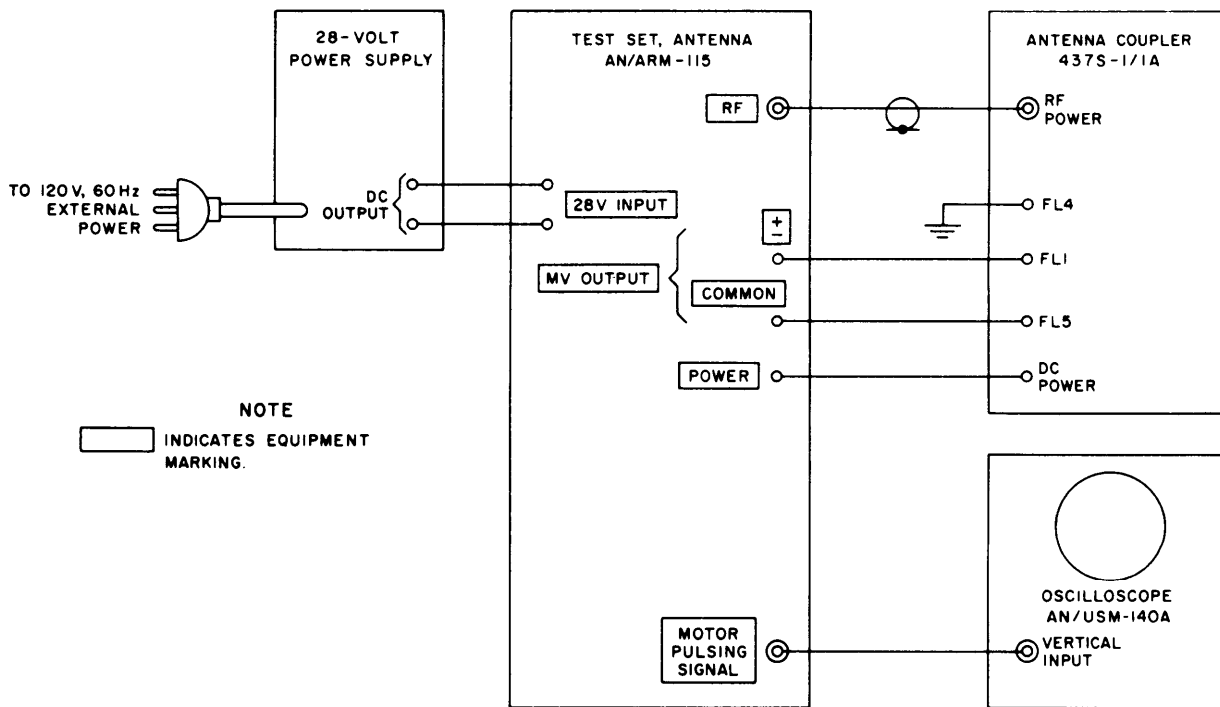
Figure 4-3. TUNE INDICATOR function test, test setup.
