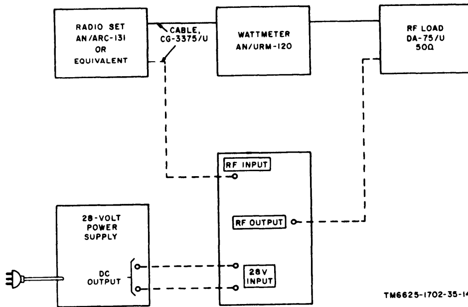
Figure 4-8. RF wattmeter test setup.
