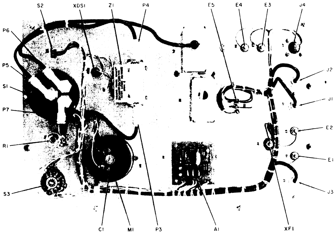
Figure 2-2. Test panel rear view, parts location.
