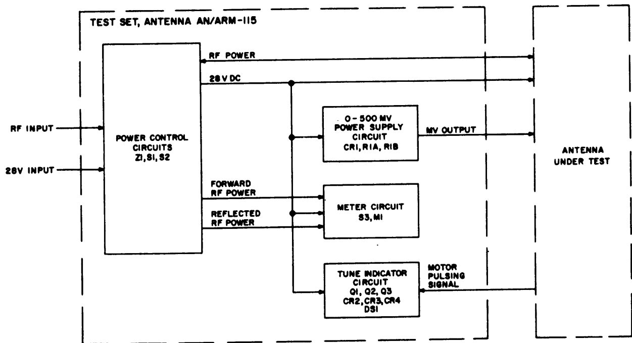
Figure 1-1. Test set, block diagram.
