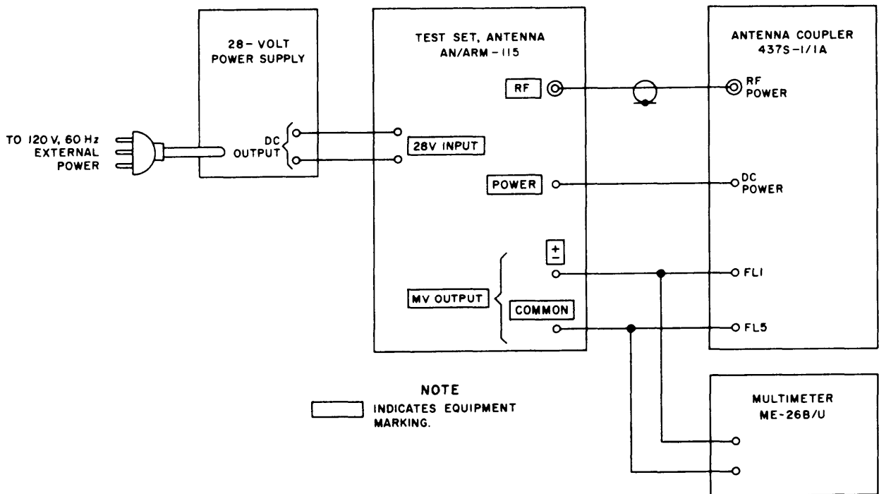
Figure 4-2. Millivolt source test, test setup.
